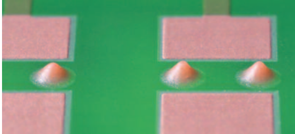
Printed PD 208 PR glue
