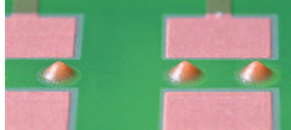
Cured PD 208 PR glue
